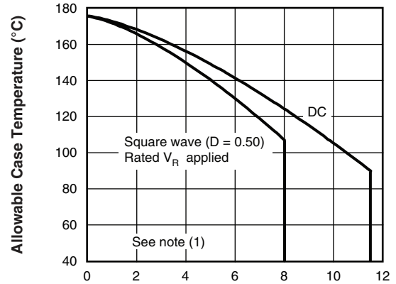
I_{F(AV)} - Average Forward Current (A) Fig. 7 - Maximum Allowable Case Temperature vs. Average Forward Current (FULL-PAK)
